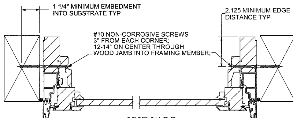
SECTION E-E SCALE 1 : 4
